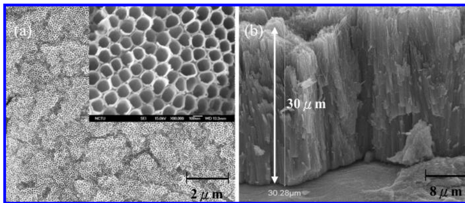
Figure 3. SEM images of ATO NT after ultrasonic cleaning: (a) top view and (b) side view. The inset of (a) shows the enlarged pattern of the ATO NT arrays.
