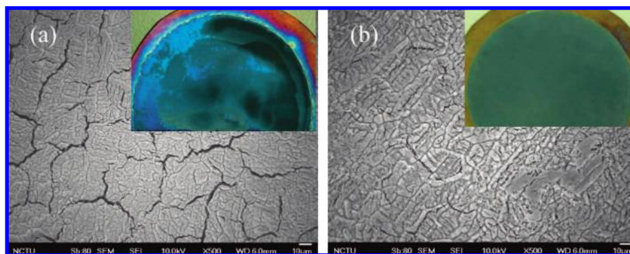
Figure 1. SEM images of ATO films undergoing (a) a one-step annealing and (b) a two-step annealing. The insets show specimen pictures of the corresponding ATO films: the one-step process leads to cracking of the films that easily peeled from the Ti substrate, whereas the two-step process yields films of satisfactory quality and ready to use.
