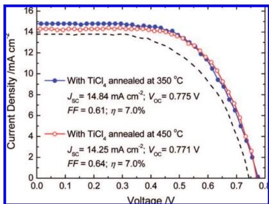
Figure 8. Current–voltage characteristics of NT-DSSC devices fabricated using the ATO films treated with TiCl 4 as shown in Figure 7 under simulated AM-1.5 solar illumination (100 mW cm -2 ) and active area 0.28 cm 2 . The dashed curve shows the results of an ATO film not treated with TiCl 4 for comparison.
