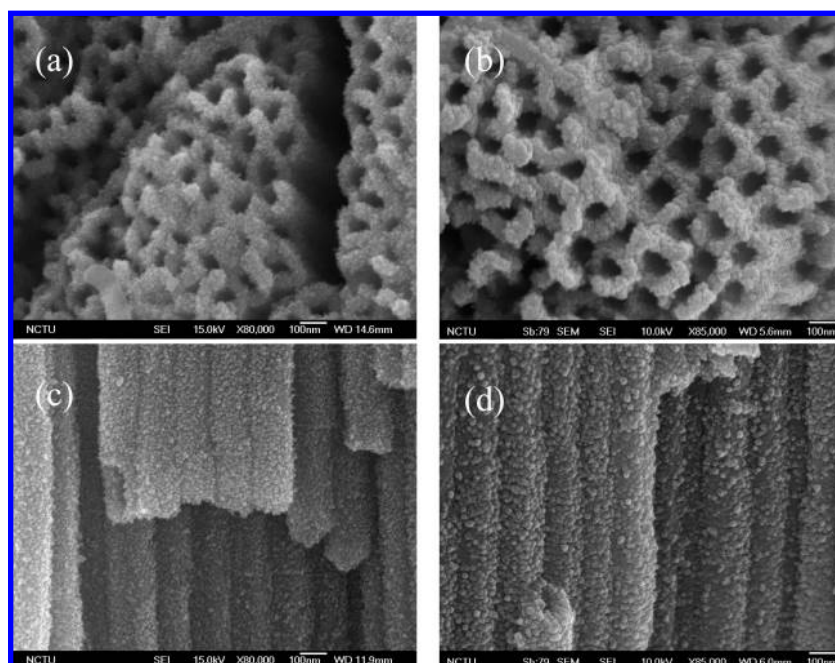
Figure 7. SEM images of ATO NT after treatments with \text{TiCl}_4 ; (a) and (c) top and side views with annealing temperature 350 \text{ }^\circ\text{C} ; (b) and (d) top and side views with annealing temperature 450 \text{ }^\circ\text{C} . The scale bars represent a length of 100 nm.
