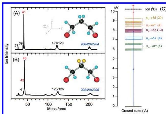
Figure 2. Femtosecond time-resolved mass spectra of (A) DBP and (B) 2,2- d 2 -DBP obtained at a delay time of \sim 50 fs. (C) Excitation/ionization scheme for the observed transient signals. All transition energies were obtained using TDDFT calculations at the B3P86/6-311++G(d,p) level, neglecting spin-orbit coupling. In parentheses we give the number for each type of the transitions involved.
