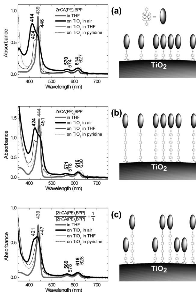
Fig. 3 Left , comparison of the absorption spectra of (a) ZnCA(PE) 1 BPP, (b) ZnCA(PE) 4 BPP, (c) 1 : 1 ZnCA(PE) 1 BPP : ZnCA(PE) 4 BPP mixture in THF (grey curves), on TiO 2 in air (bold solid curves), on TiO 2 in THF (thin solid curves), on TiO 2 in pyridine (dotted curves). Right , schematic presentation of the porphyrin assembly on nanocrystalline TiO 2 surfaces. Note that the lengths of the porphyrins and the diameter of TiO 2 particles are scaled accordingly ( \sim 1 – 3 nm for the porphyrin lengths and \sim 20 nm for the of TiO 2 particle diameters). Since only very small amounts of the porphyrins are allowed to adsorb onto these TiO 2 films, the right schemes depict part of the spherical surface of an individual TiO 2 particle partially covered by the porphyrins.
