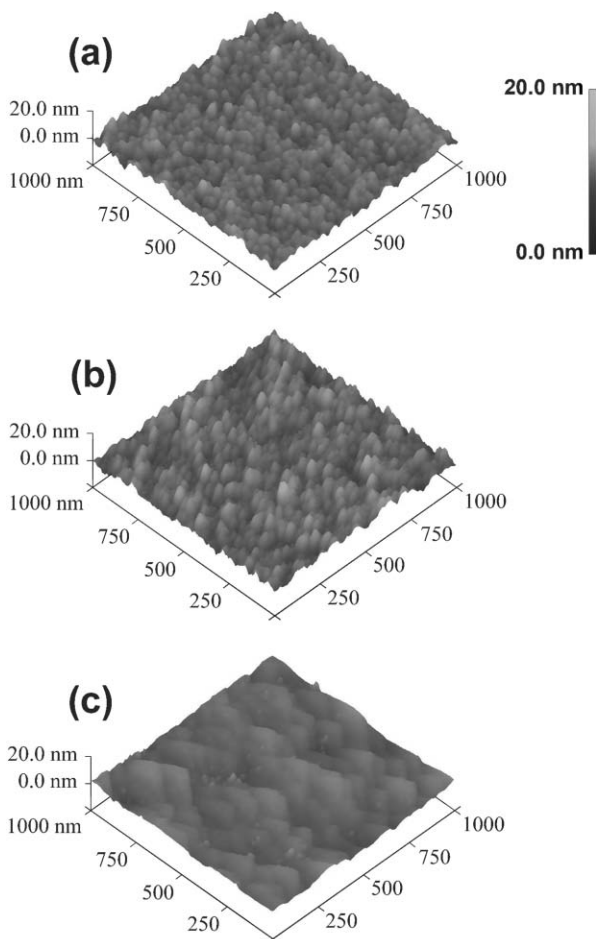
Fig. 2 AFM images of (a) bare TiO 2 , (b) ZnCA(PE) 1 BPP/TiO 2 , and (c) ZnCA(PE) 4 BPP/TiO 2 (spin-coated TiO 2 films). Mean roughness: (a) 12 nm, (b) 13 nm, and (c) 10 nm. Note that the triangular features in (c) are suggested to be TiO 2 aggregates. The small dots in (c) have diameters of 14–40 nm, consistent with the sizes of TiO 2 particles observed in (a).
