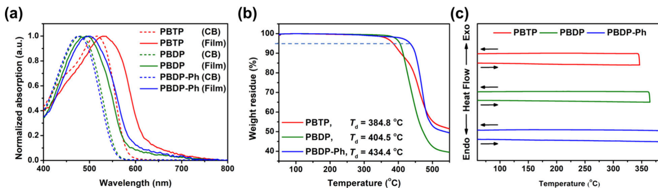
Figure 2. Normalized absorption spectra (a) of PBTP, PBDDP, and PBDDP-Ph in CB and thin films, (b) TGA and (c) DSC measurements of PBTP, PBDDP, and PBDDP-Ph with a ramping rate of 10 °C/min.
