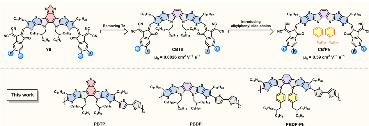
Figure 1. Chemical structures showing Y6, CB16, and CB'Ph nonfullerene acceptors as well as PBTP, PBDP, and PBDP-Ph polymers reported in this work.
