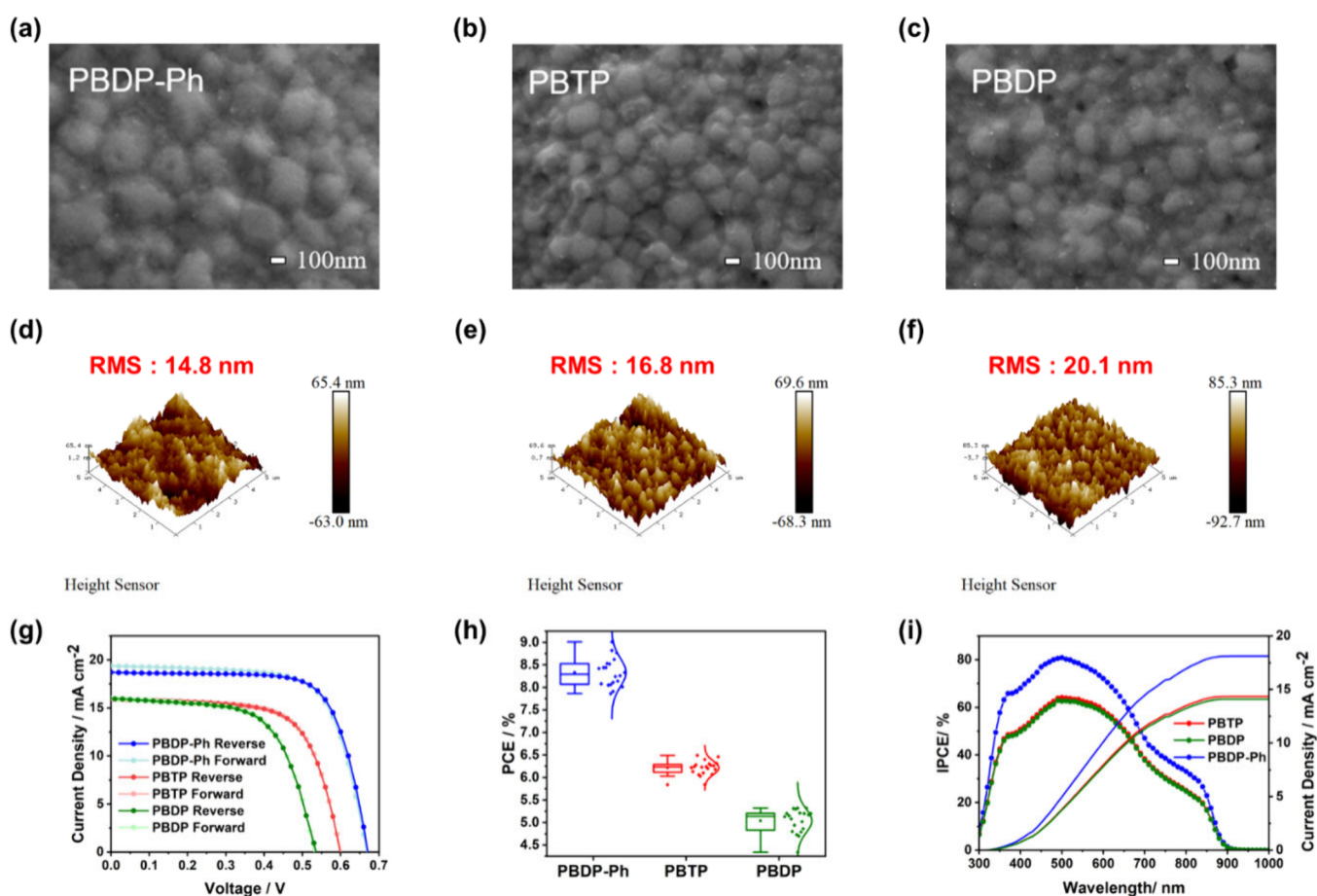
Figure 5. (a–c) Top-view SEM images of Sn-based perovskite films deposited on PBDP-Ph , PBTP , and PBDP HTLs. (d–f) Three-dimensional AFM images of Sn-based perovskite films fabricated on PBDP-Ph , PBTP , and PBDP HTLs. (g) J – V curves of TPSCs employing different polymer HTLs. (h) Statistical distribution of PCEs of 20 devices based on different HTLs. (i) IPCE spectra and the corresponding integrated current densities of TPSCs incorporating various HTLs.
