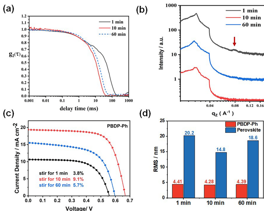
Figure 3. (a) DLS autocorrelation functions g_2(\tau) of PBBDP-Ph in toluene solutions stirred for 1, 10, and 60 min. (b) GI-SAXS profiles of spin-coated PBBDP-Ph films processed from the 1-, 10-, and 60 min stirring solutions. (c) J-V curves of PBBDP-Ph-based TPSCs using polymer solutions stirred for different durations. (d) Comparison of AFM root-mean-square (RMS) surface roughness of PBBDP-Ph polymer films (1, 10, and 60 min), and the corresponding perovskite layers deposited on top of the polymer HTLs.
